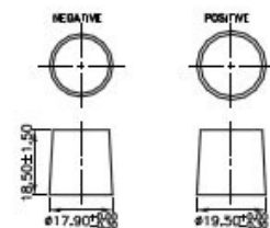
TERMINAL DETAIL
