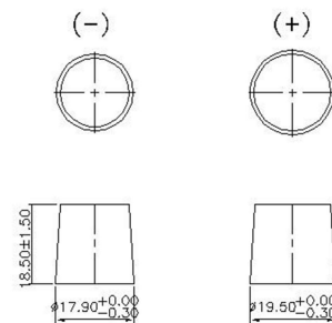
POST TERMINAL DETAIL
